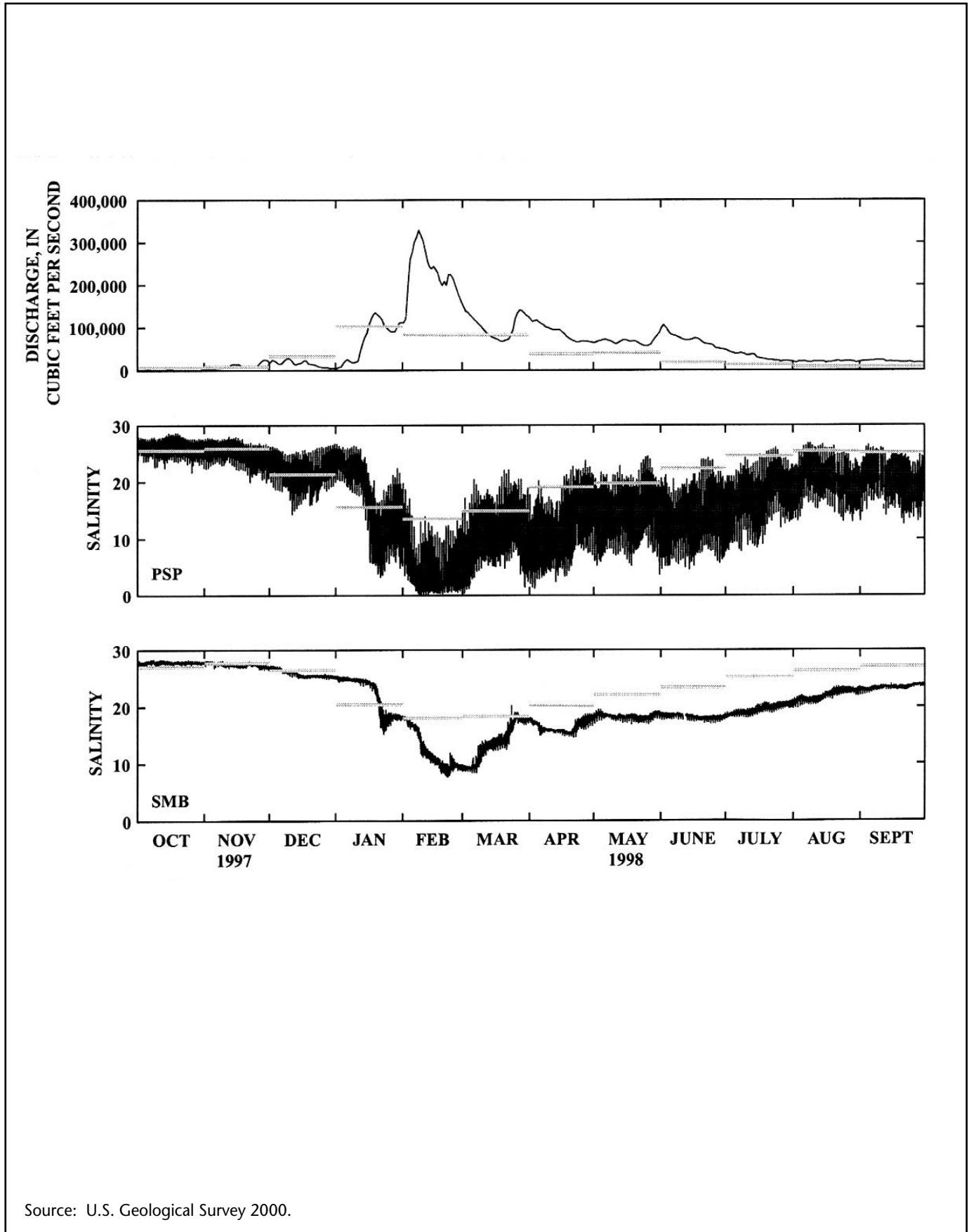
Figure 4-1 Time Series of Delta Outflow and Salinity at Point San Pablo and San Mateo Bridge – Water Year 1998
