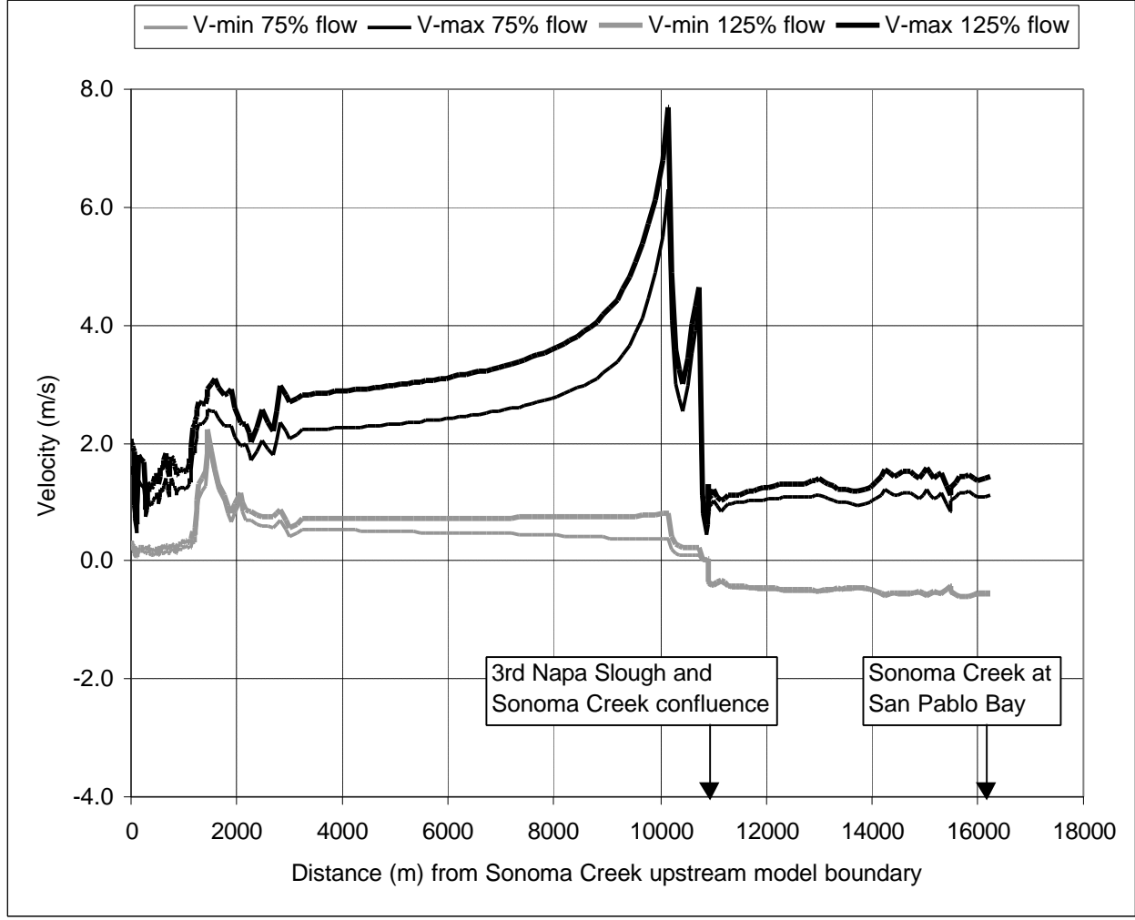
figure 3 Sonoma Creek Velocity Sensitivity to Discharge Boundary Condition Source: 1411-12 #
