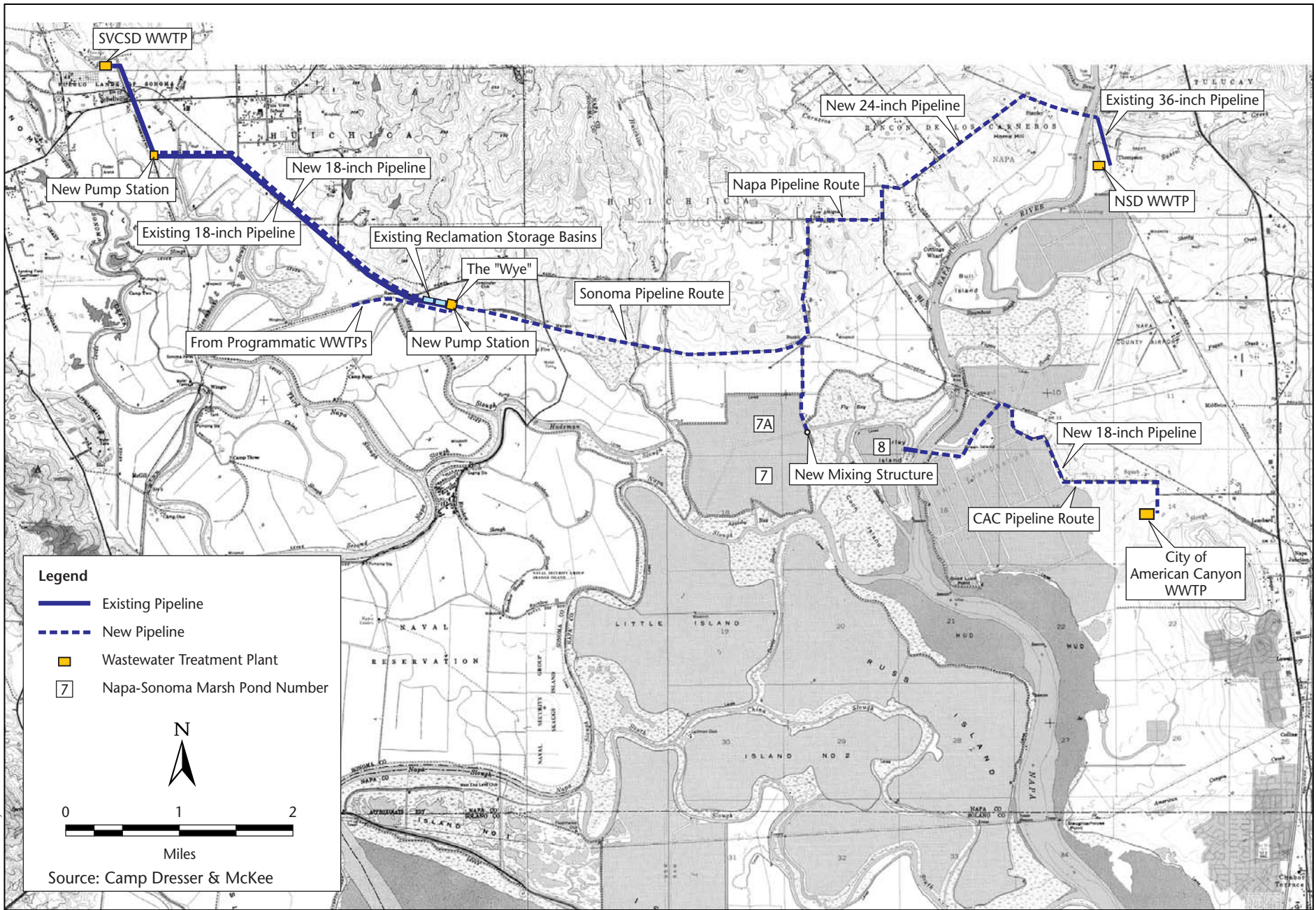
Figure 4-7 Recycled Water Delivery
